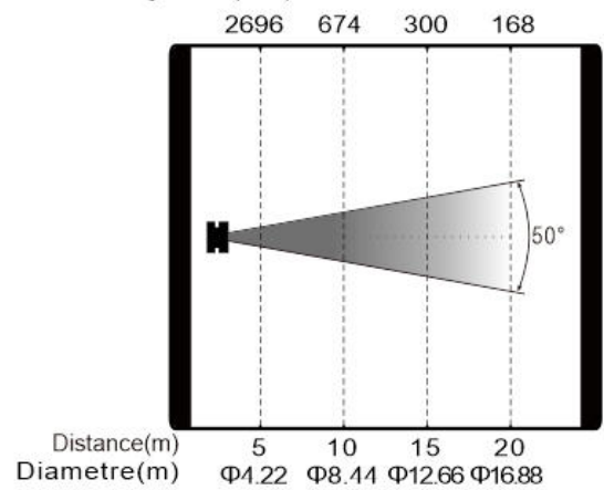
SL5000PH Pro Max. Beam Mode Intensity LUX (50°)
