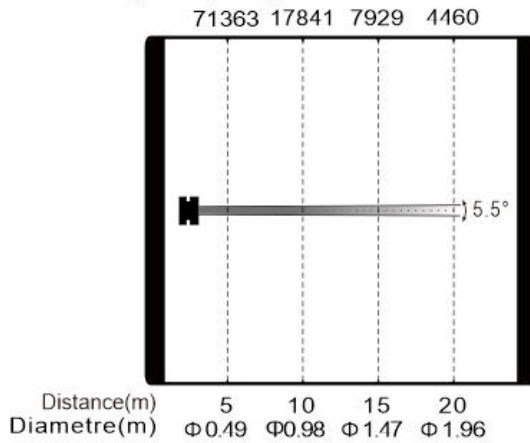
SL5000PH Pro Min. Beam Mode Intensity LUX (5.5 °)
