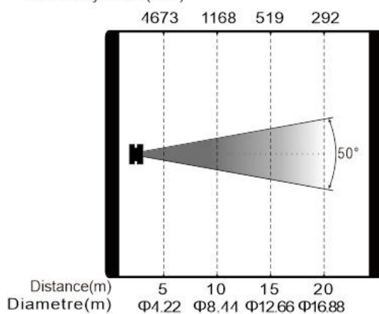
SL5000PH Ultra Max. Beam Mode Intensity LUX (50°)
