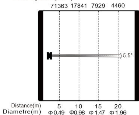
SL5000PH Ultra Min. Beam Mode Intensity LUX (5.5 °)
