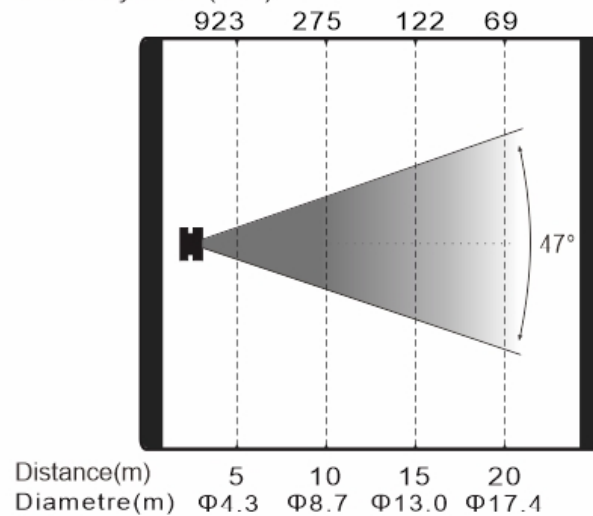
Intensity LUX (47°)
