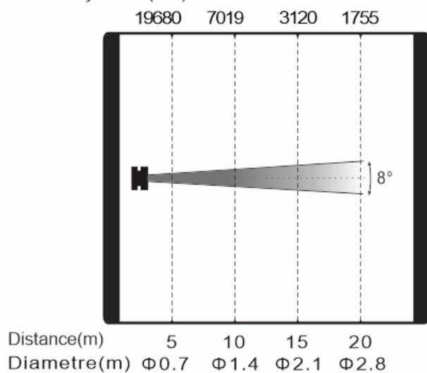
Intensity LUX (8 °)
