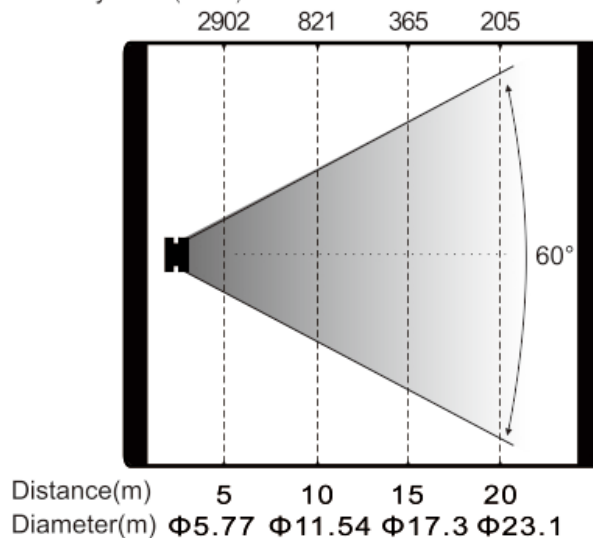
Intensity LUX (60° )
