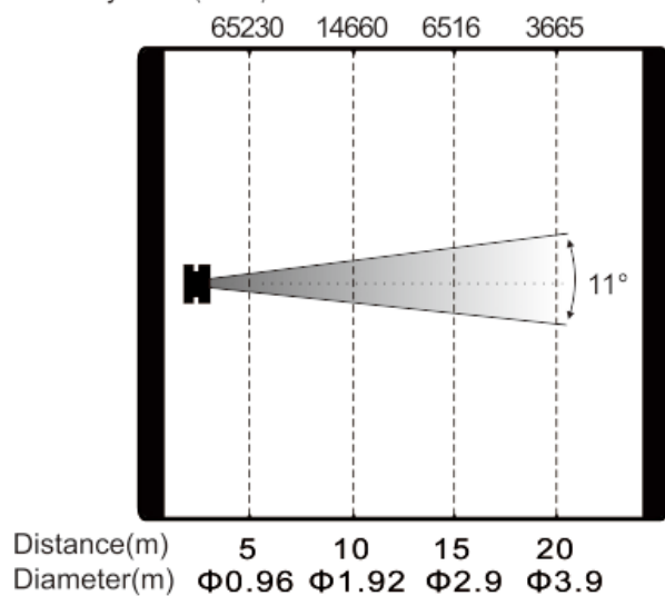
Intensity LUX (11° )
