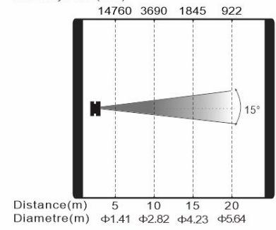
Max. Wash Mode Intensity LUX (15°)
