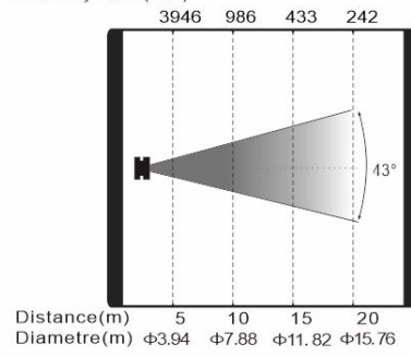
Max. Spot Mode Intensity LUX (43°)
