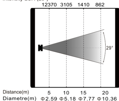
Max. Beam Mode Intensity LUX (29°)
