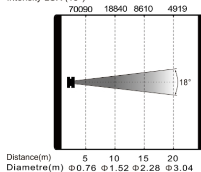
Min. Wash Mode Intensity LUX (18°)
