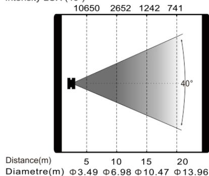
Max. Spot Mode Intensity LUX (40°)
