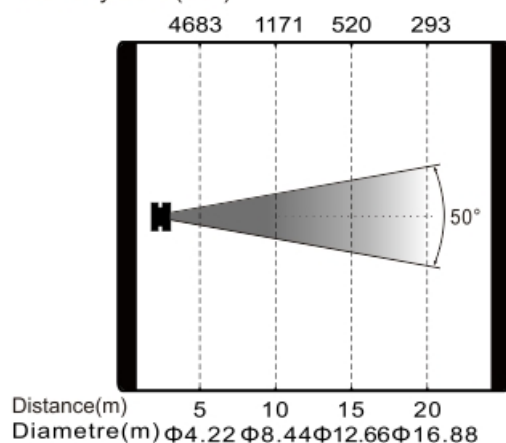
SL5000P IP Max. Beam Mode Intensity LUX (50°)
