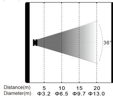
T90H IP (WW) Intensity LUX (36°)
