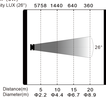
T90H IP (WW) Intensity LUX (26°)
