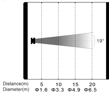
T90H IP (WW) Intensity LUX (19°)
