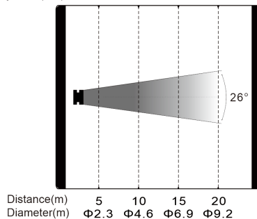
T90H IP (WW) Intensity LUX (26°)
