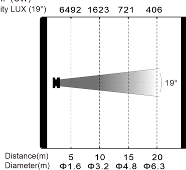
T90H IP (WW) Intensity LUX (19°)
