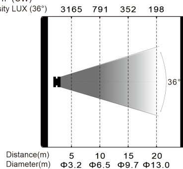
T90H IP (WW) Intensity LUX (36°)
