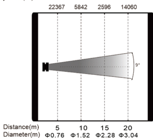
Intensity LUX (9°)
