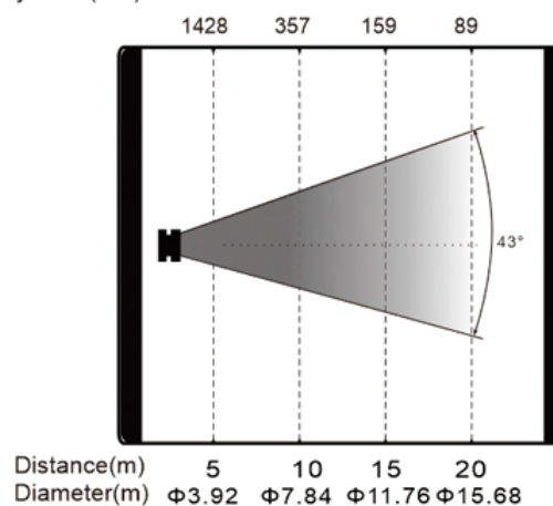
Intensity LUX (43°)
