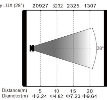
Max.Beam Mode Intensity LUX (28°)
