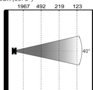
Max. Wash Mode Intensity LUX (39.5°)
