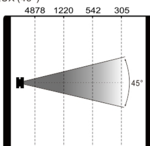
Max. Spot Mode Intensity LUX (45°)
