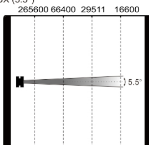
Min. Spot Mode Intensity LUX (5.5°)
