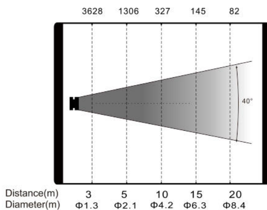
Intensity LUX(40°)
