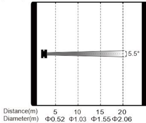
SL15PH IP Pro Min.Field angle Intensity LUX (5.5°) 78500 21000 9345 5250
