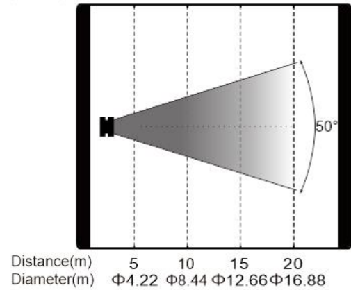
SL15PH IP Pro Max.Field angle Intensity LUX (50°) 3675 861 410 231
