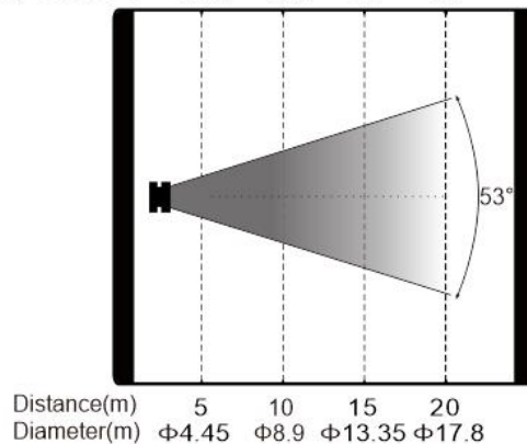
(SL750PH Pro) Max. Beam angle
