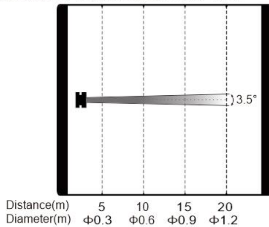
SL880P IP Pro Intensity LUX (3.5°) 106800 26700 11870 6675
