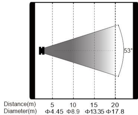
SL880PH IP Pro Intensity LUX (53°) 1200 300 133 75
