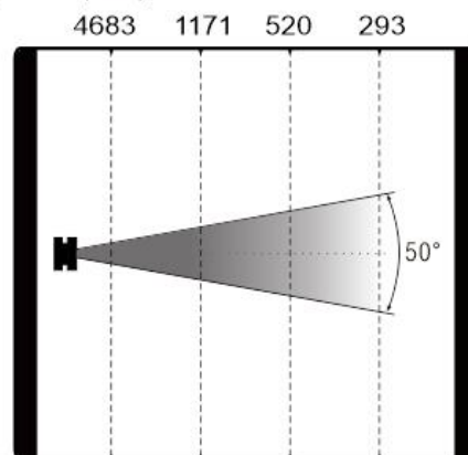
SL5000P IP Pro Max. Beam angle Intensity LUX (50°)
