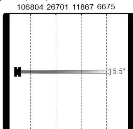
SL5000P IP Pro Min. Beam angle Intensity LUX (5.5°)
